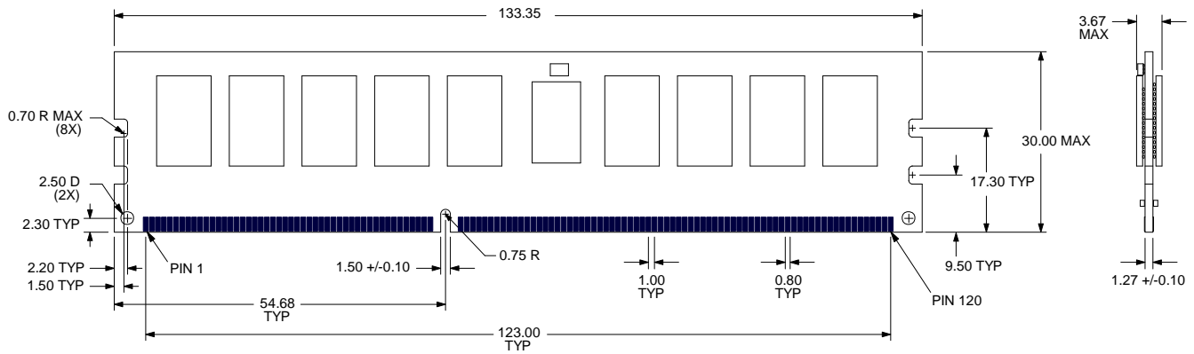
BACK VIEW
